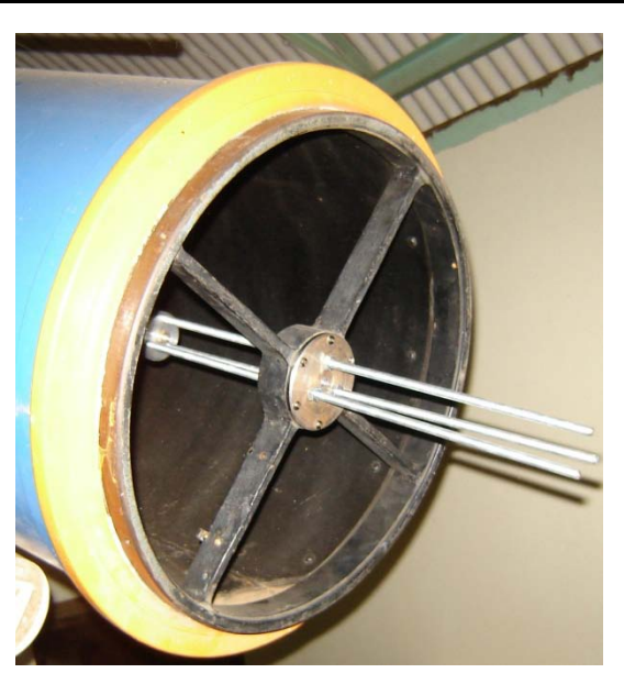
Newtonian secondary optics
